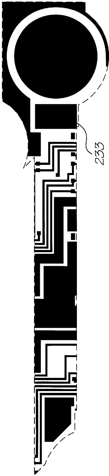
Metal 2 mask
