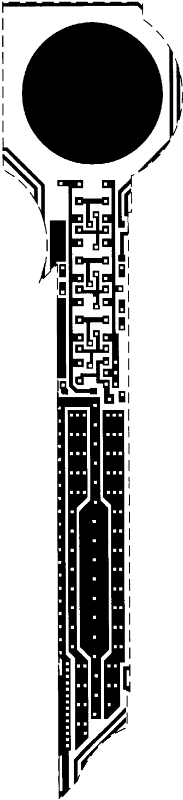
Metal 1 mask
