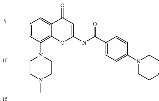
N-[8-(4-Methyl-piperazin-1-yl)-4-oxo-4H-chromen-2-yl]-4-morpholin-4-yl-benzamide
