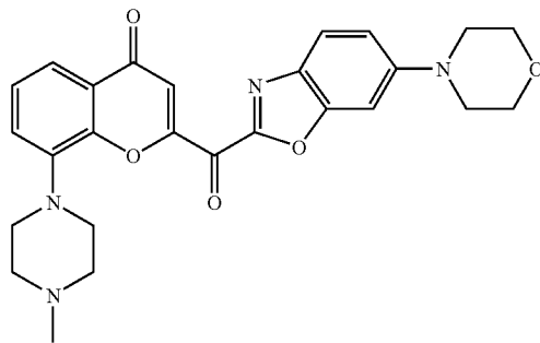
8-(4-Methyl-piperazin-1-yl)-2-(6-morpholin-4-yl-benzooxazol-2-yl)-chromen-4-one
