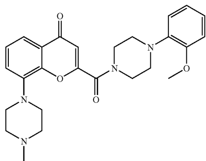
2-{1-[4-(2-Methoxy-phenyl)-piperazin-1-yl]-methanoyl}-8-(4-methyl-piperazin-1-yl)-chromen-4-one
