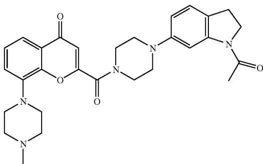
2-{1-[4-(1-Acetyl-2,3-dihydro-1H-indol-6-yl)-piperazin-1-yl]-methanoyl}-8-(4-methyl-piperazin-1-yl)-chromen-4-one
