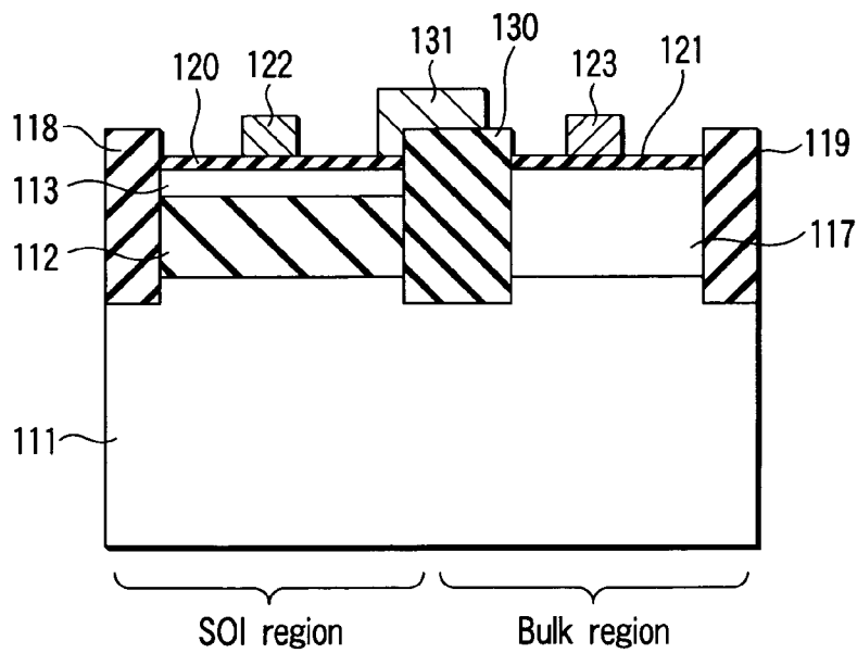
FIG. 47 PRIOR ART
