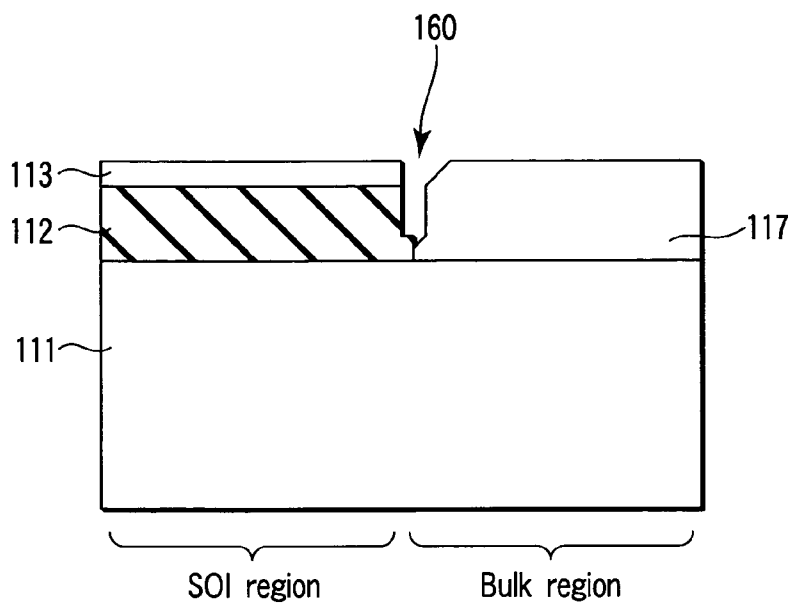
FIG. 46 PRIOR ART
