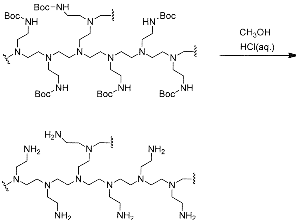
Reaction scheme 2
