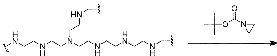
15 Reaction scheme 1
