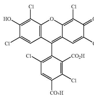
5-carboxy-HEX
