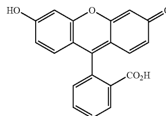
Fluorescein
