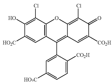
JOE
