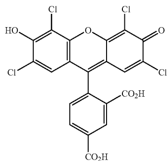
ZOE
