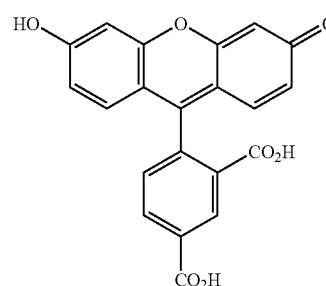
5-carboxyfluorescein
