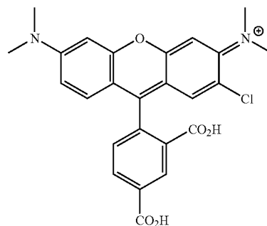
5-carboxyrhodamine
