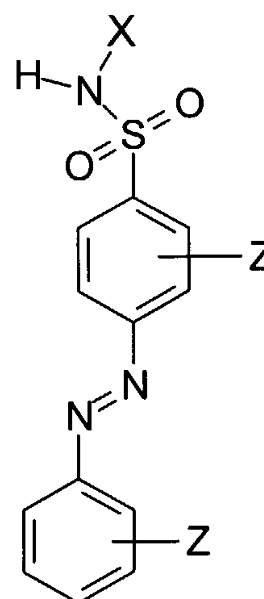
Dabsyl
