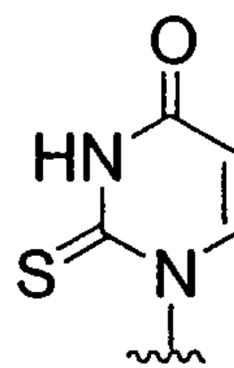
2-thio-Uracil
