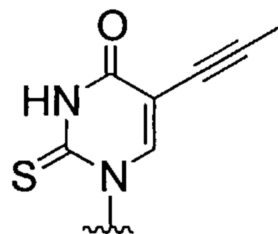
2-thio-5-propynyl-Uracil
