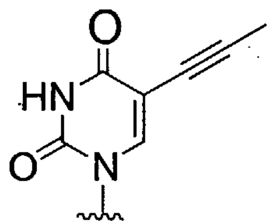
5-propynyl-Uracil
