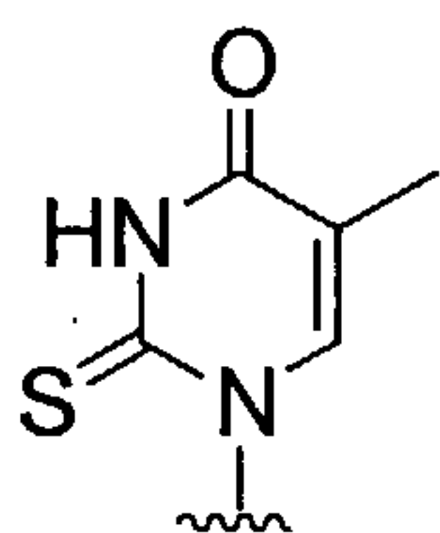
2-thio-Thymine
