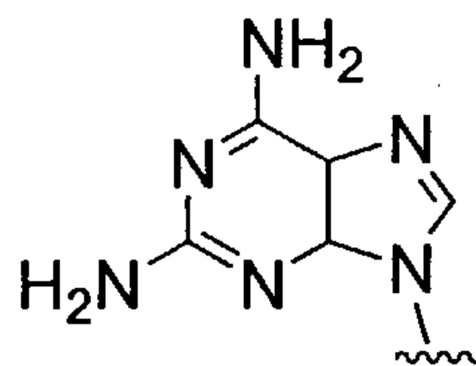
N9-(2,6,-diaminopurine)
