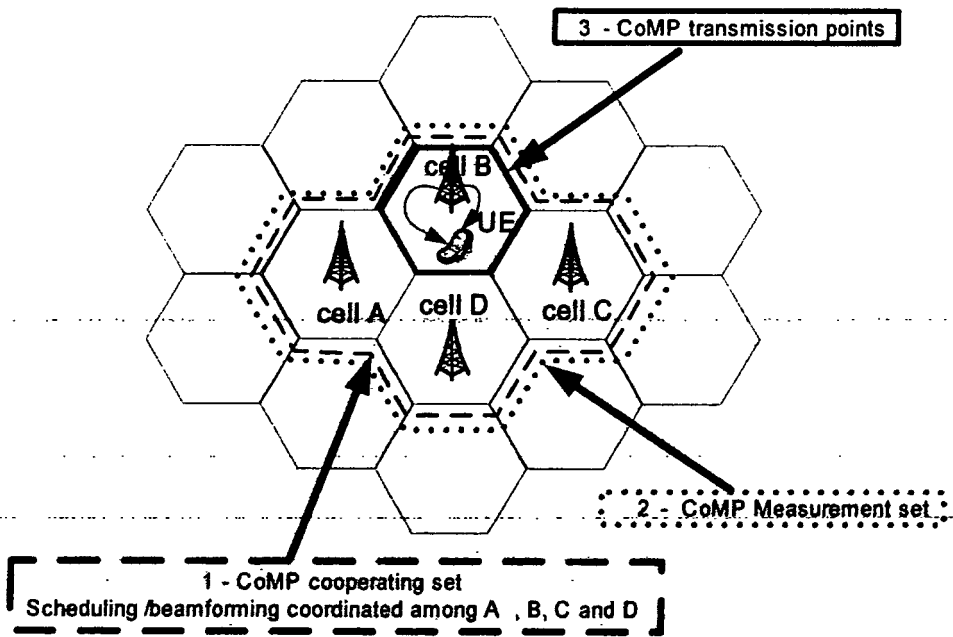
(b) CoMP CS/CB
