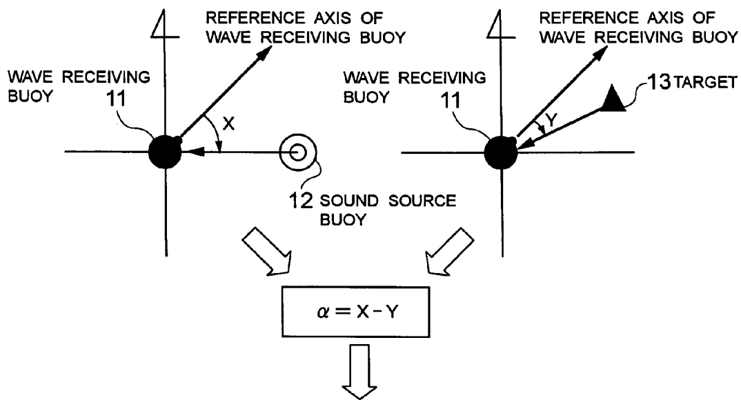
FIG. 5C TRANSITION DIAGRAM (GPS)
