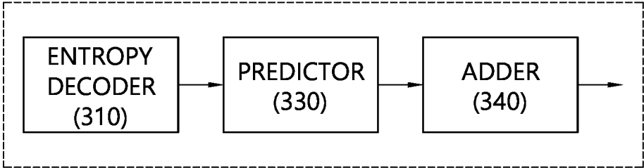
DECODING APPARATUS
