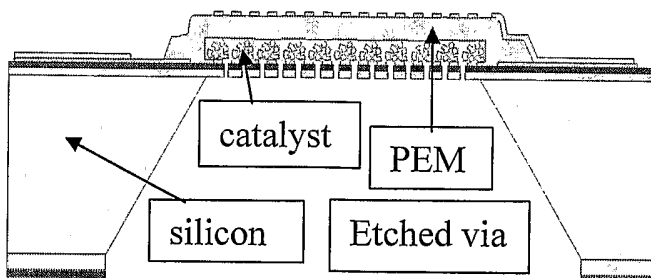
Apply and pattern upper electrode
