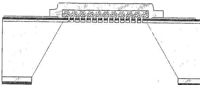
Apply PEM layer such as by spinning.
