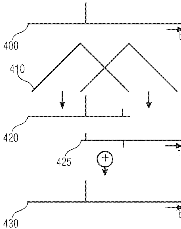
FIGURE 4 (PRIOR ART)
