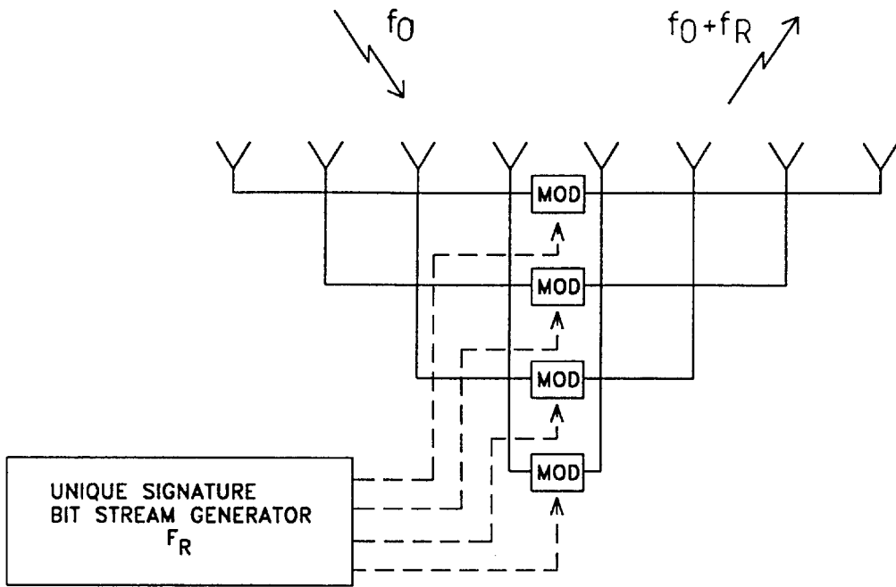
FIG 4 (Prior Art)
