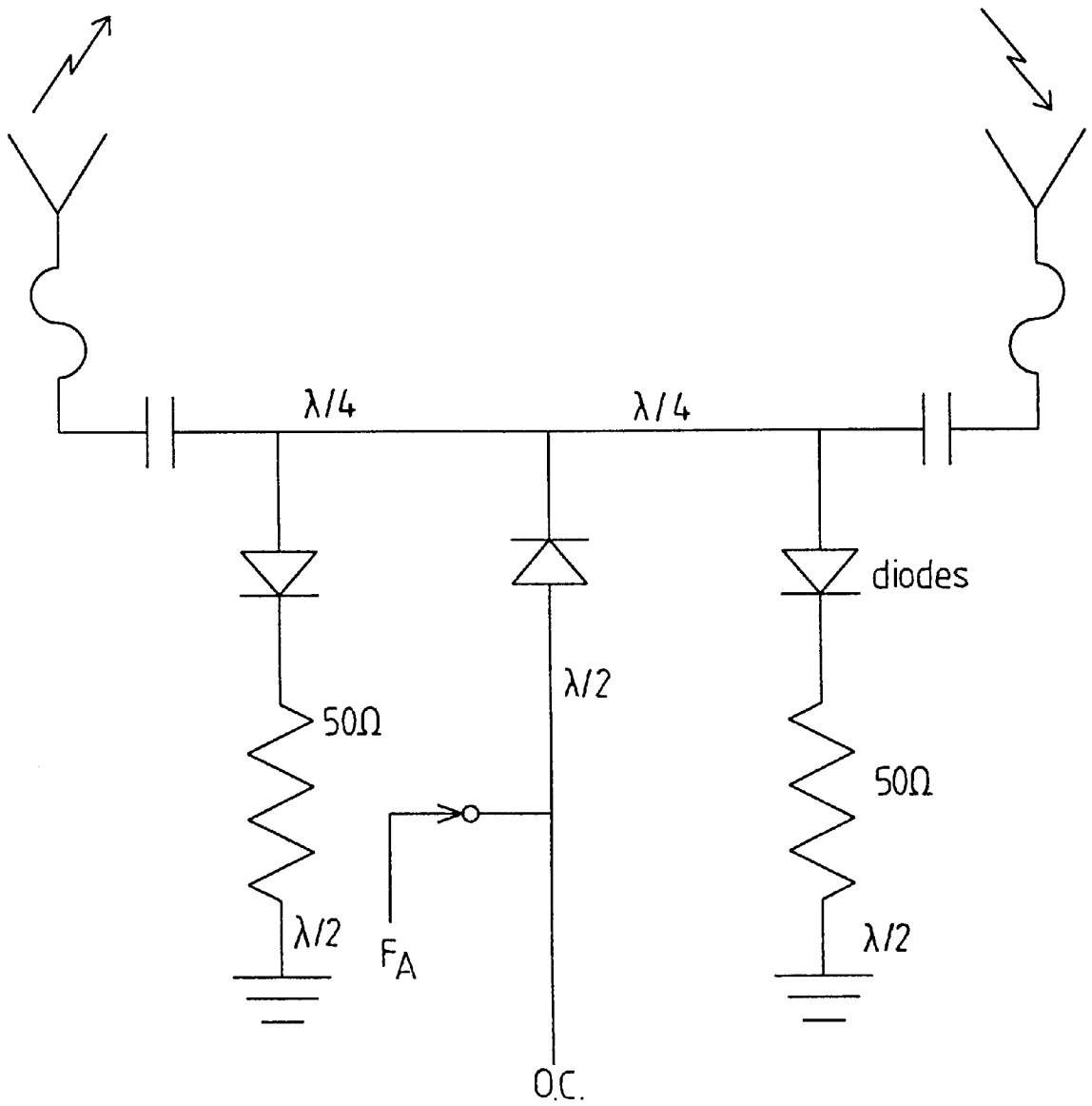
FIG 1 (Prior Art)
