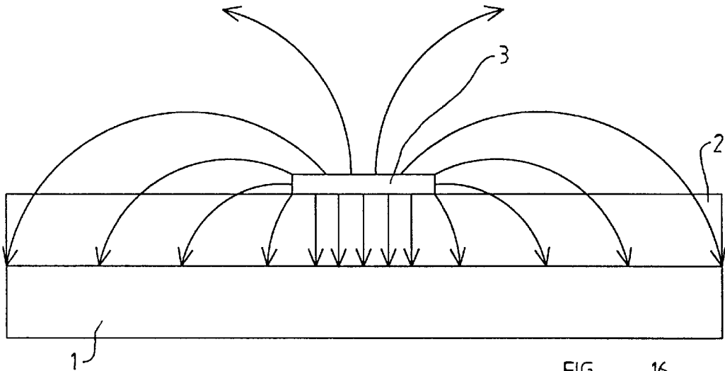
FIG 16 (Prior Art)
