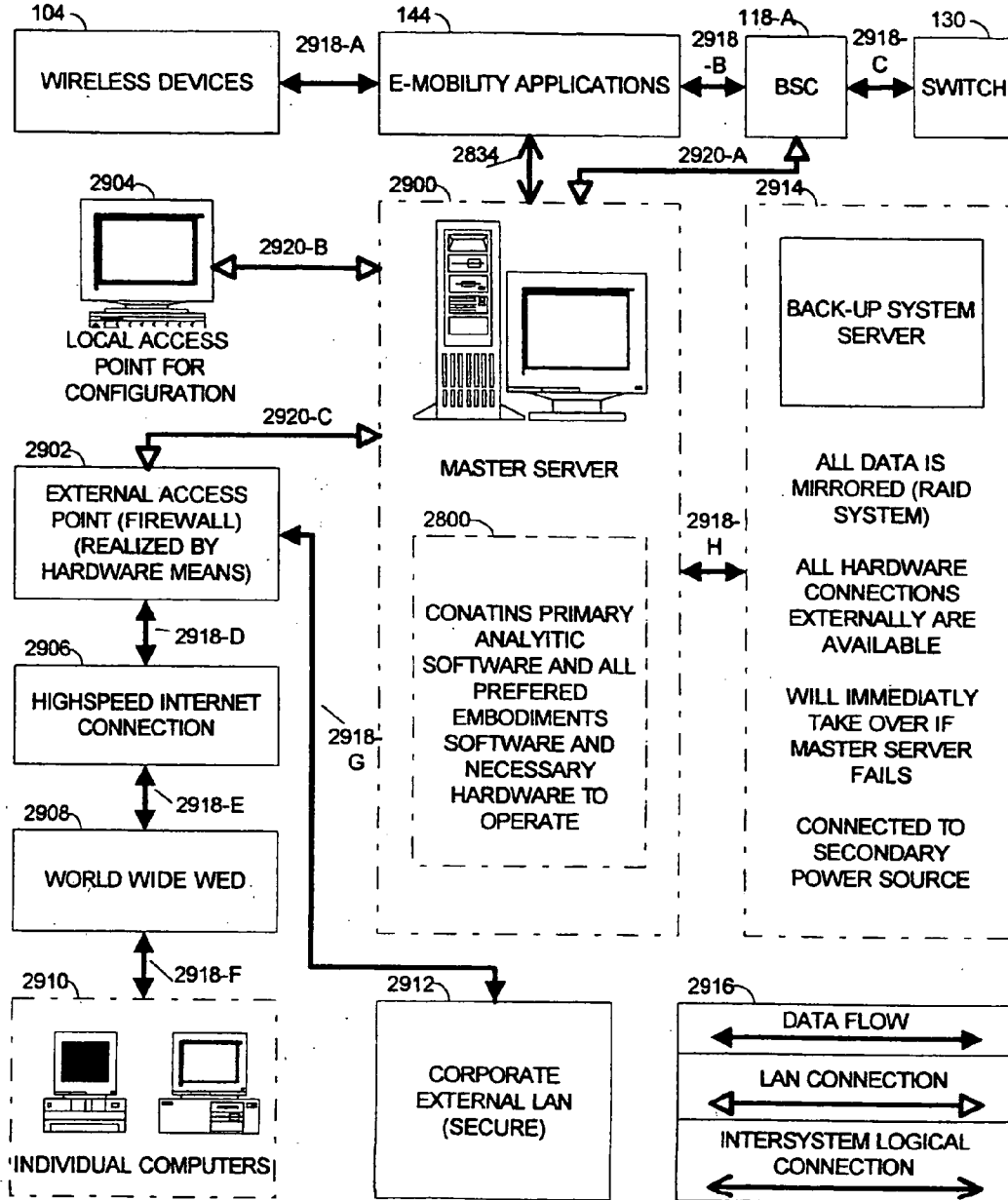
PHYSICAL REALIZATION OF PREFERRED EMBODIMENTS FIG. 29
