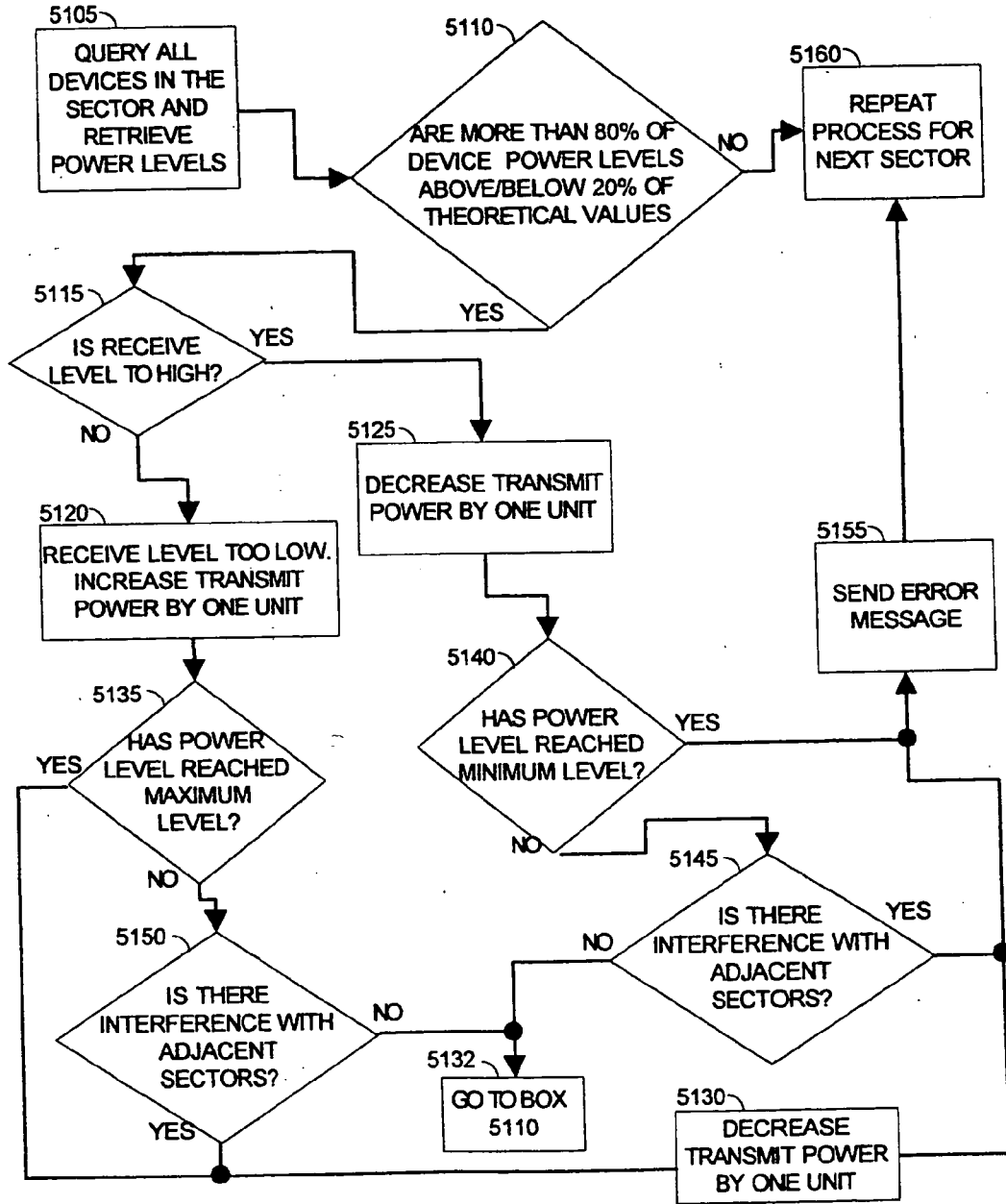
NETWORK EQUIPMENT TUNING FLOWCHART
