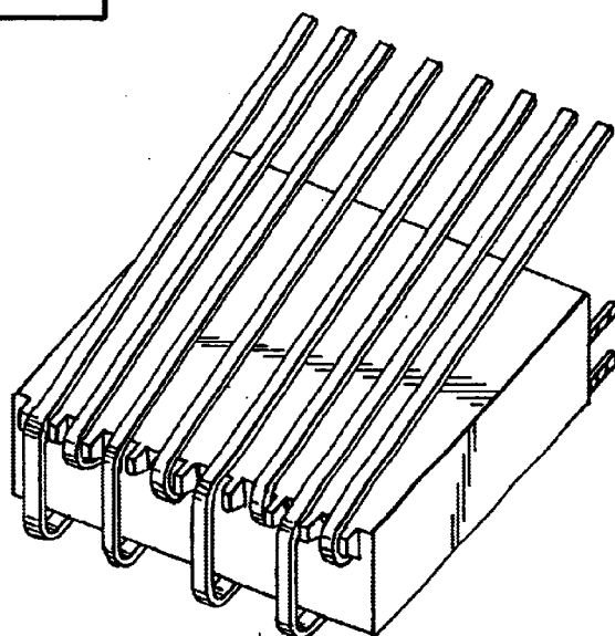
Figure 8 (Prior Art)
