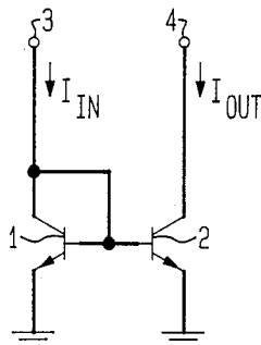
FIG. 1 (PRIOR ART)
