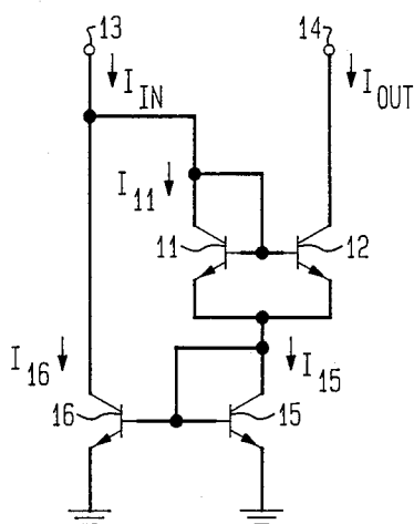
FIG. 2 (PRIOR ART)
