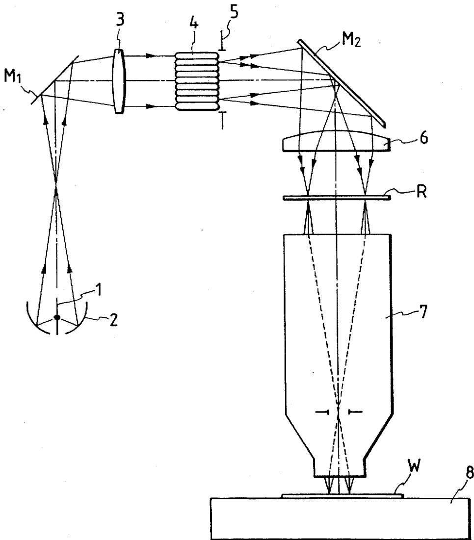
FIG. 12 PRIOR ART
