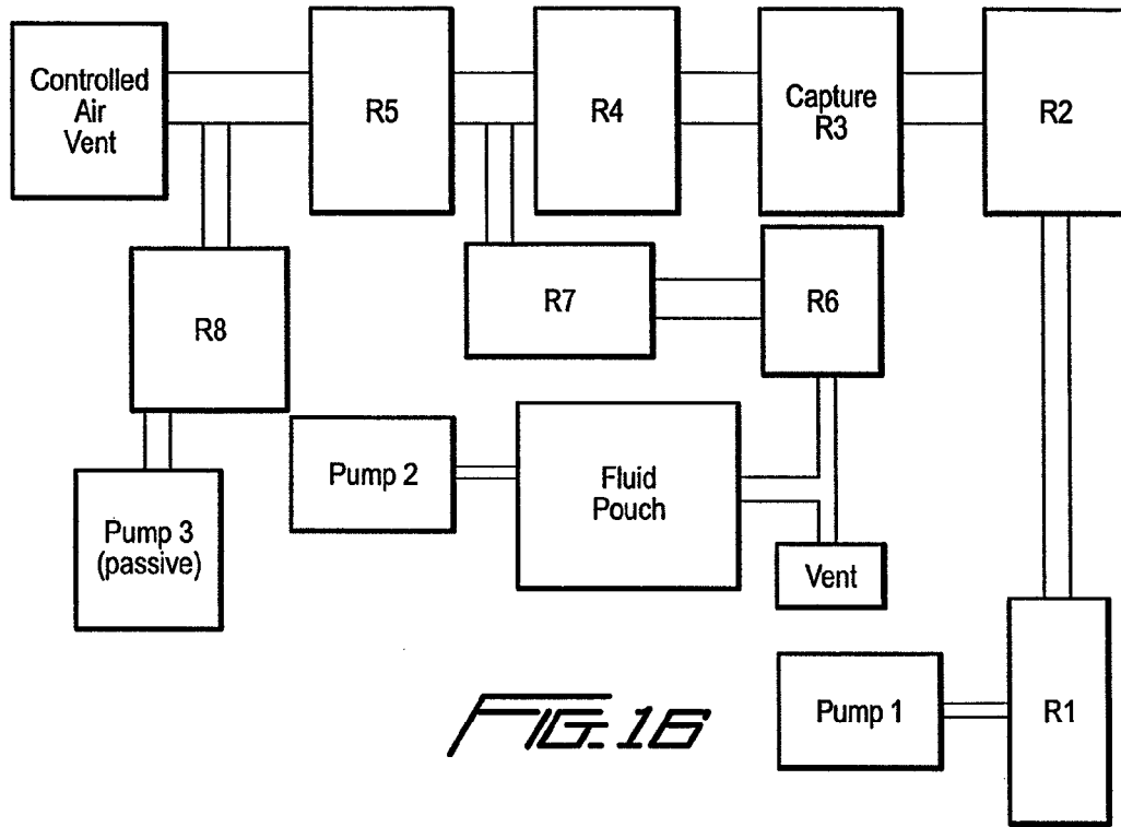
Fluidic Schematic for i-STAT immunocartridge
