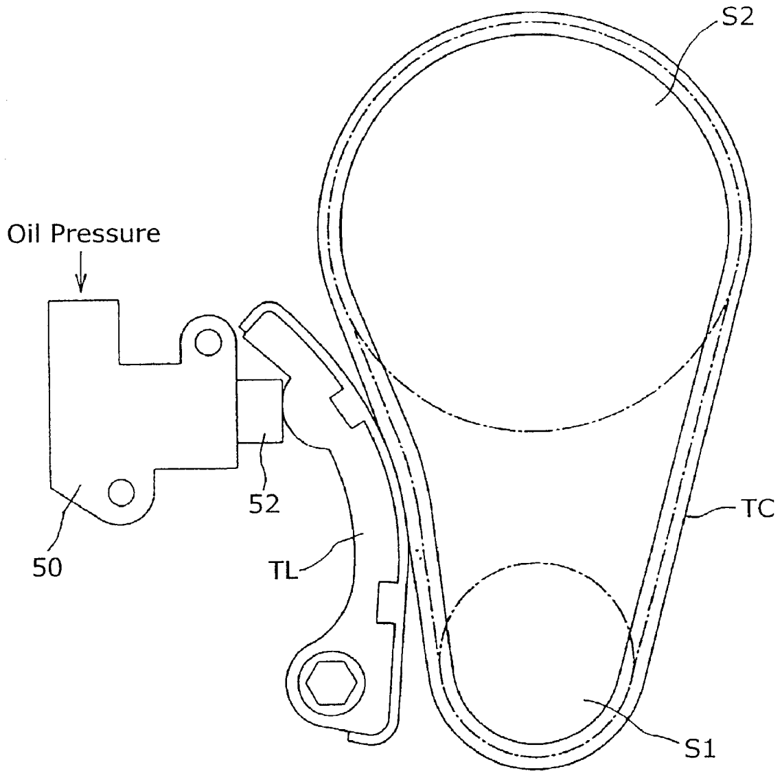
Fig.9 Prior Art
