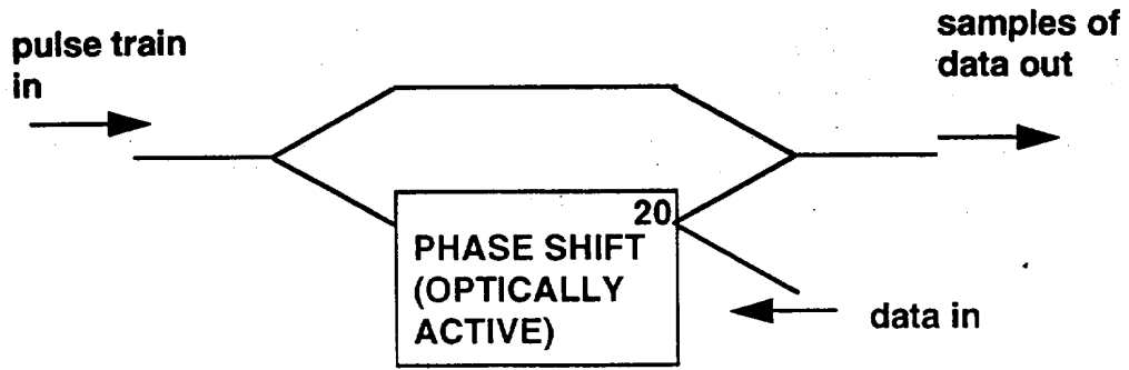
Fig 3 INTERFEROMETER ARRANGEMENT
