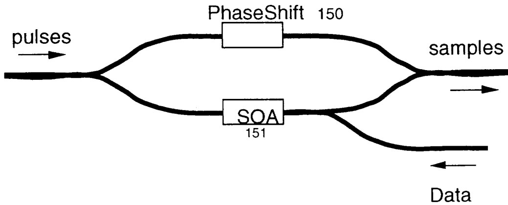
Fig 19 Interferometer Arrangement
