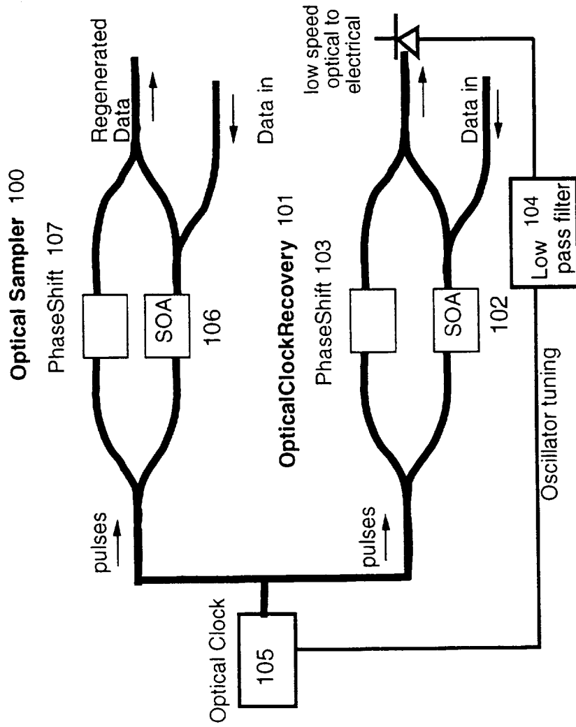
Fig 12 Optical Regenerator
