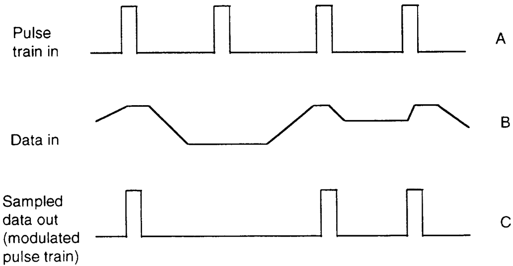
Fig 4 INTERFEROMETER OPERATING AS SAMPLER
