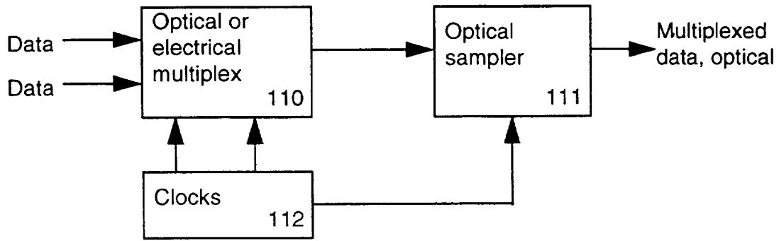
Fig 13 MULTIPLEXER
