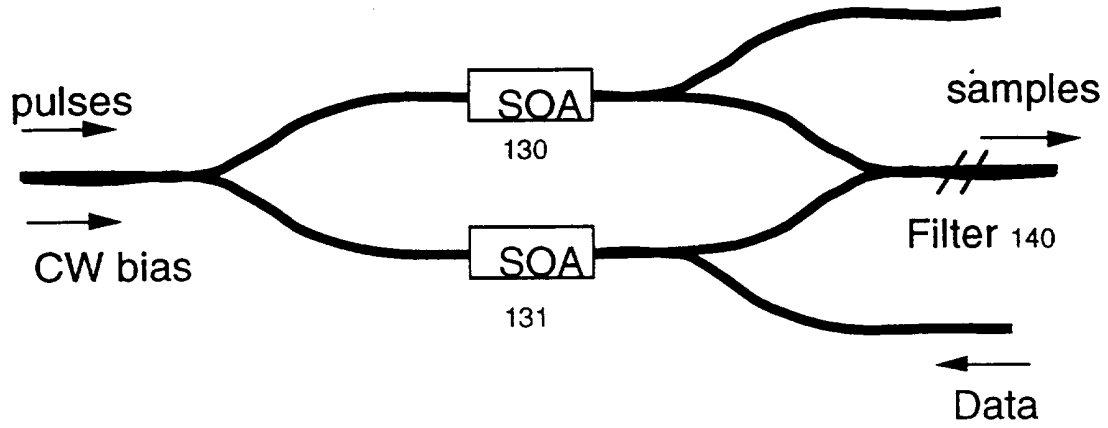
Fig 18 Interferometer Arrangement
