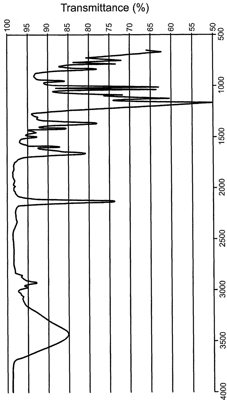
Wavenumber (cm -1 )
