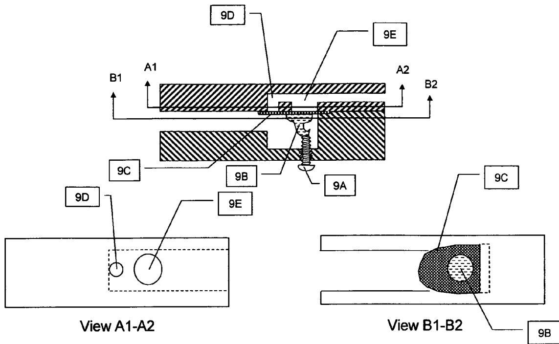
Figure 2A Second Valve Assembly (expanded, without shank)
