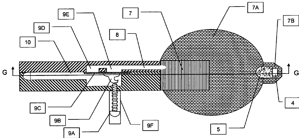
Figure 2B Complex Single Unit
