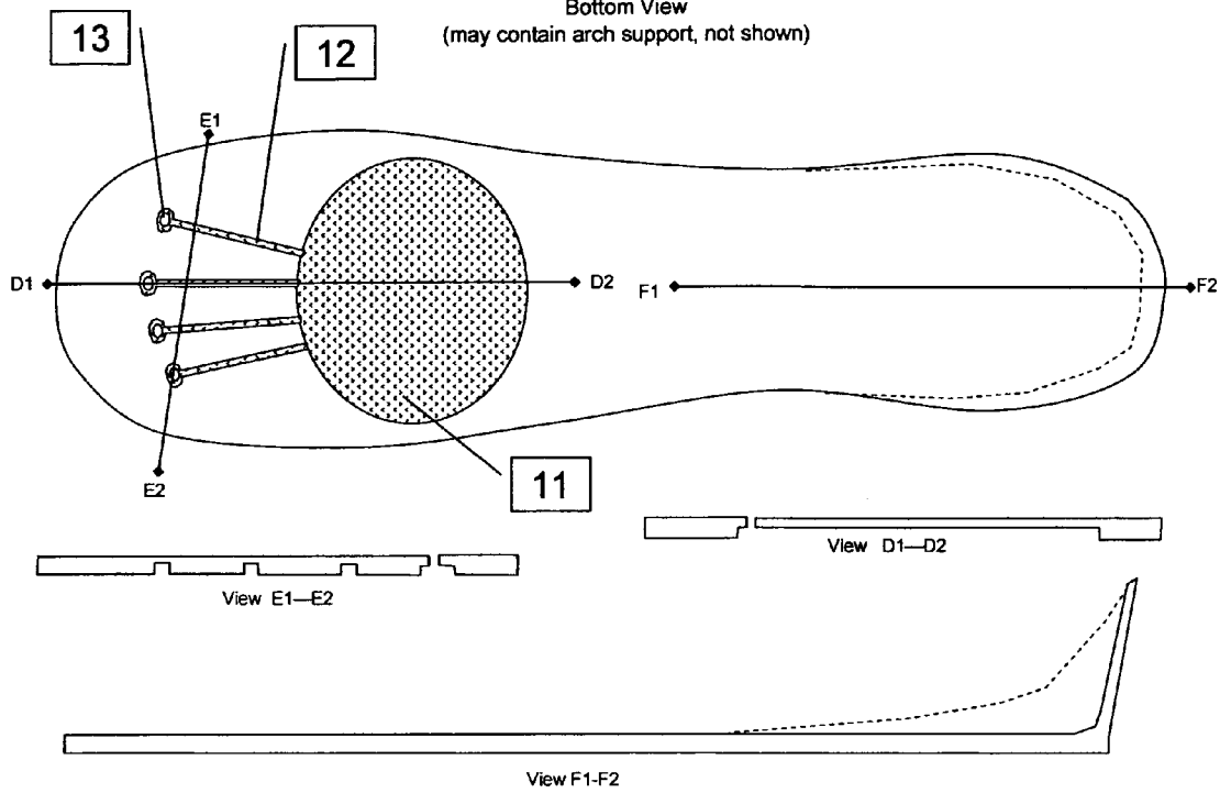
Figure 4 Shoe Liner
