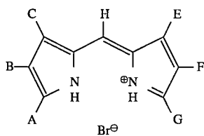
Dipyrromethenes
