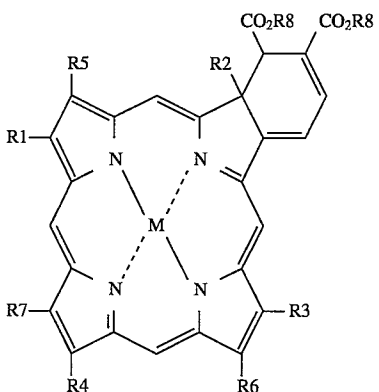
Formula 4
