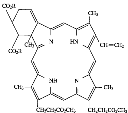
Adduct IX
