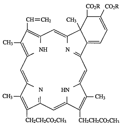
Adduct VIII
