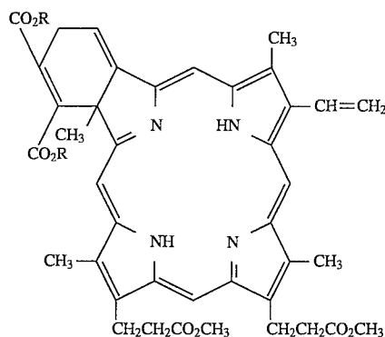
Adduct V
