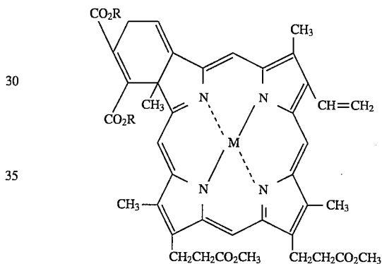
Complex V
