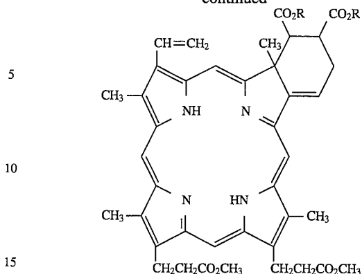
Adduct X
