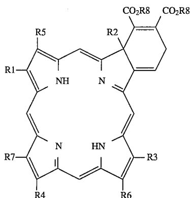
Formula 9
