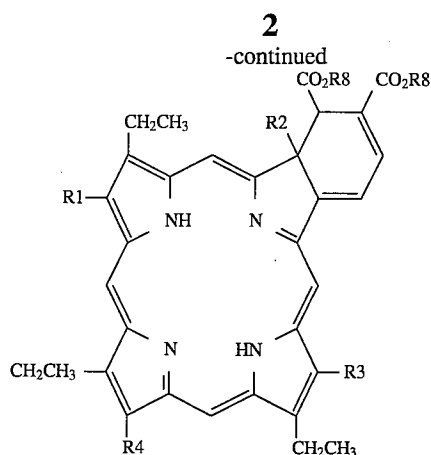
Formula 2
