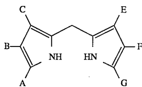
Dipyrromethanes
