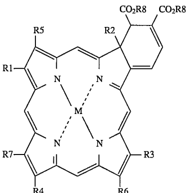
Formula 12
