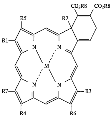
Formula 11
