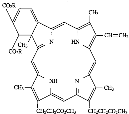
Adduct VII
