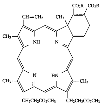
Adduct VI
