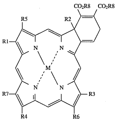
Formula 3
