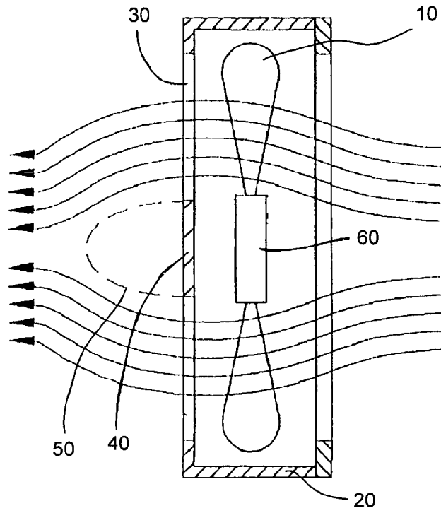
Fig. 3 (prior art)
