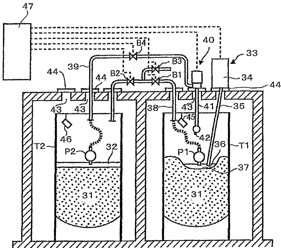
FIG. 11 Prior Art
