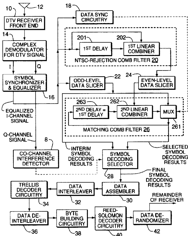
ONE OF 1ST & 2ND LINEAR COMBINERS IS A SUBTRACTOR & THE OTHER IS AN ADDER
