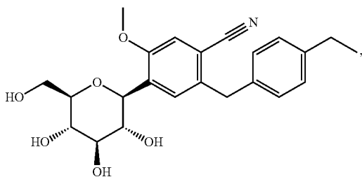
2-(4-ethylbenzyl)-4-(β-D-glucopyranos-1-yl)-5-methoxybenzonitrile
