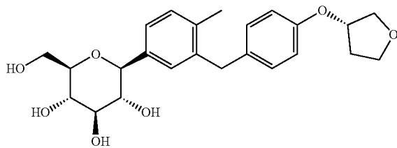
1-methyl-2-[4-((S)-tetrahydrofuran-3-yloxy)benzyl]-4-(β-D-glucopyranos-1-yl)benzene
