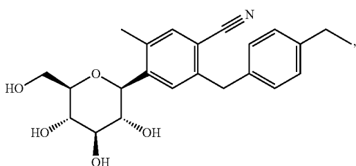
1-cyano-2-(4-ethylbenzyl)-4-(β-D-glucopyranos-1-yl)-5-methylbenzene
