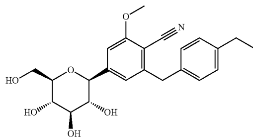
6-(4-ethylbenzyl)-4-(β-D-glucopyranos-1-yl)-2-methoxybenzonitrile
