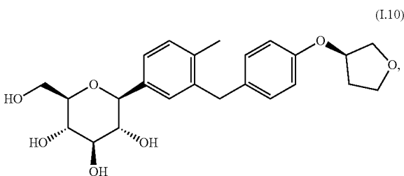
1-methyl-2-[4-((R)-tetrahydrofuran-3-yloxy)-benzyl]-4-(β-D-glucopyranos-1-yl)-benzene
