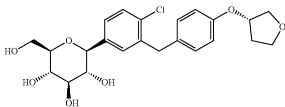
1-chloro-4-(β-D-glucopyranos-1-yl)-2-[4-((S)-tetrahydrofuran-3-yloxy)benzyl]benzene
