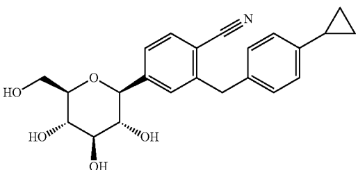
2-(4-cyclopropylbenzyl)-4-(β-D-glucopyranos-1-yl)-benzonitrile
