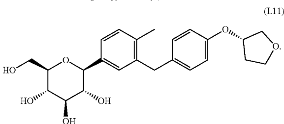
1-methyl-2-[4-((S)-tetrahydrofuran-3-yloxy)-benzyl]-4-(β-D-glucopyranos-1-yl)-benzene
