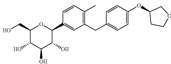
1-methyl-2-[4-((R)-tetrahydrofuran-3-yloxy)benzyl]-4-(β-D-glucopyranos-1-yl)benzene
