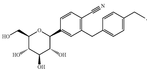
2-(4-cyclopropylbenzyl)-4-(β-D-glucopyranos-1-yl)-benzonitrile
