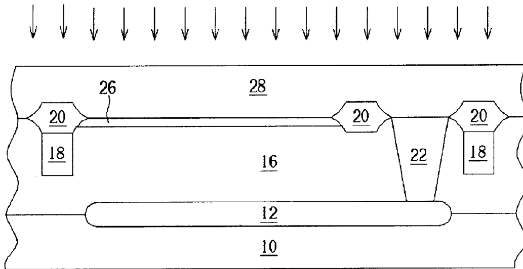
Fig. 5 Prior art
