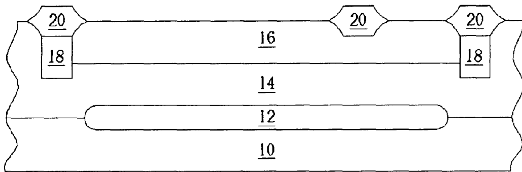
Fig. 2 Prior art
