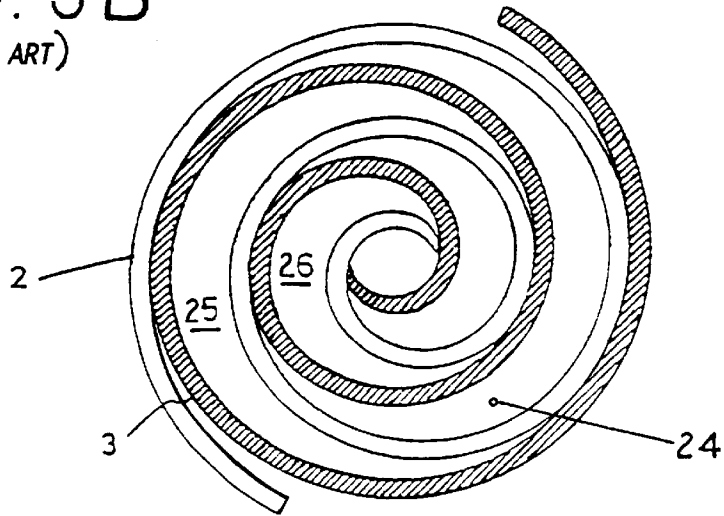
FIG. 3C (PRIOR ART)
