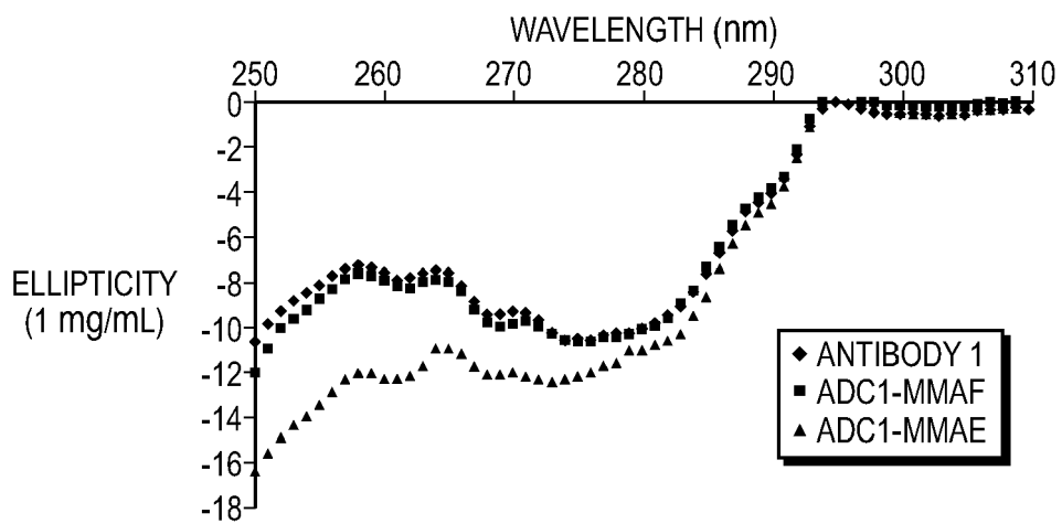
NEAR UV CD FIG. 4B
