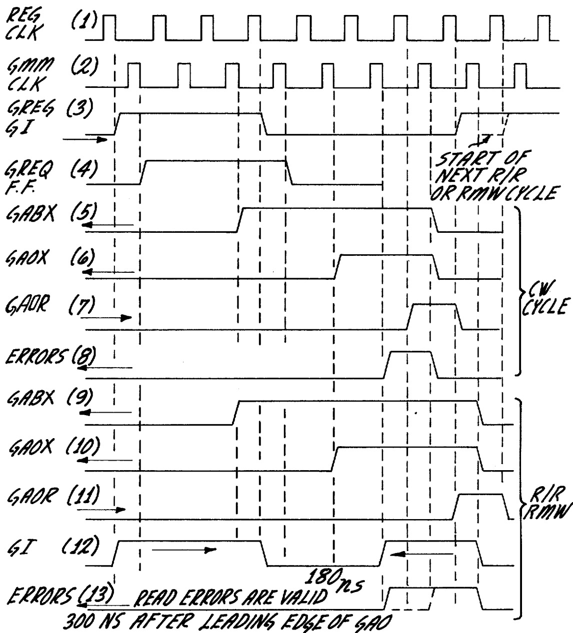
FIG. 20 TIMING RELATIONSHIPS
