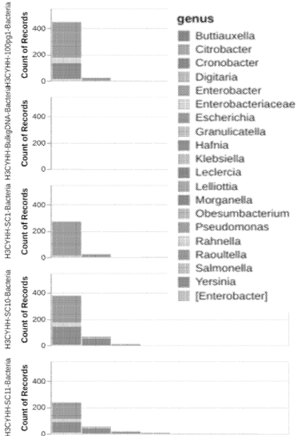
Representative genus assignments of contigs > 5KB
