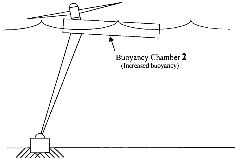
Figure 3 Turbine in Maintenance Position
