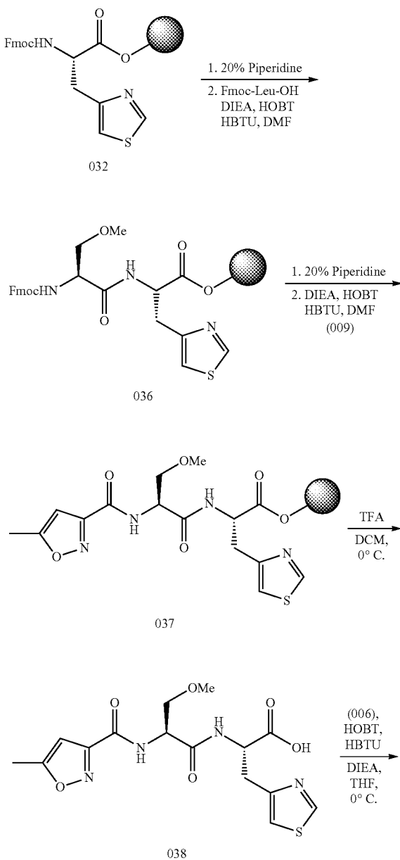
Scheme 5: Synthesis of Example 039
