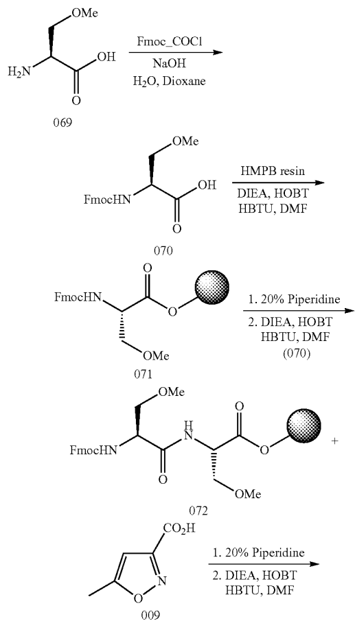
Scheme 11: Synthesis of Example 075 (approach A)
