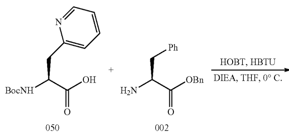
Scheme 8: Synthesis of Example 055
