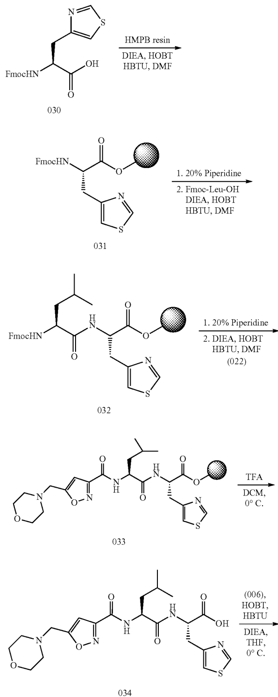
Scheme 4: Synthesis of Example 035
