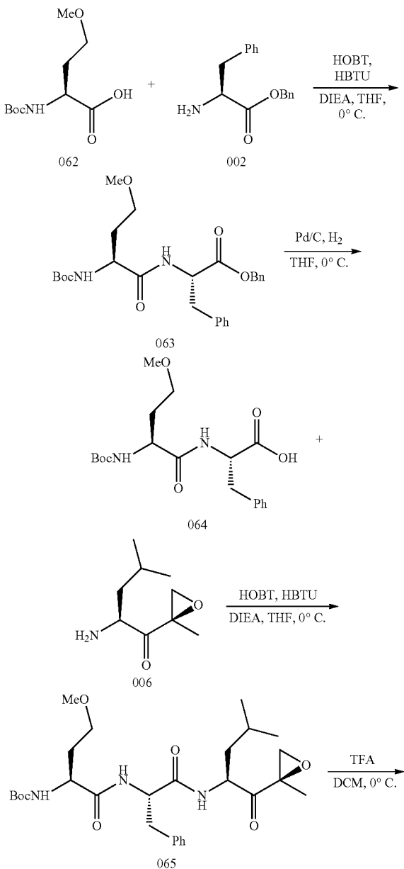
Scheme 10: Synthesis of Example 068
