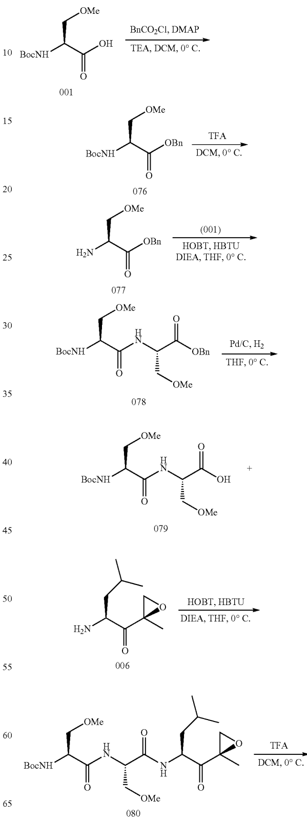
Scheme 12: Synthesis of Example 075 (approach B)
