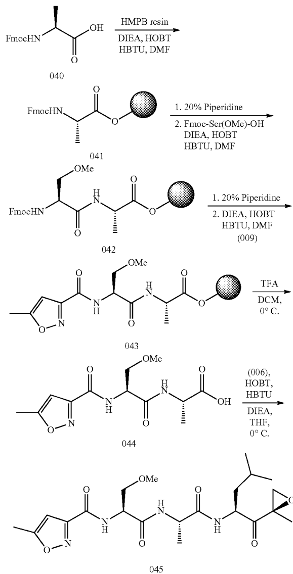
Scheme 6: Synthesis of Example 045 (approach A)
