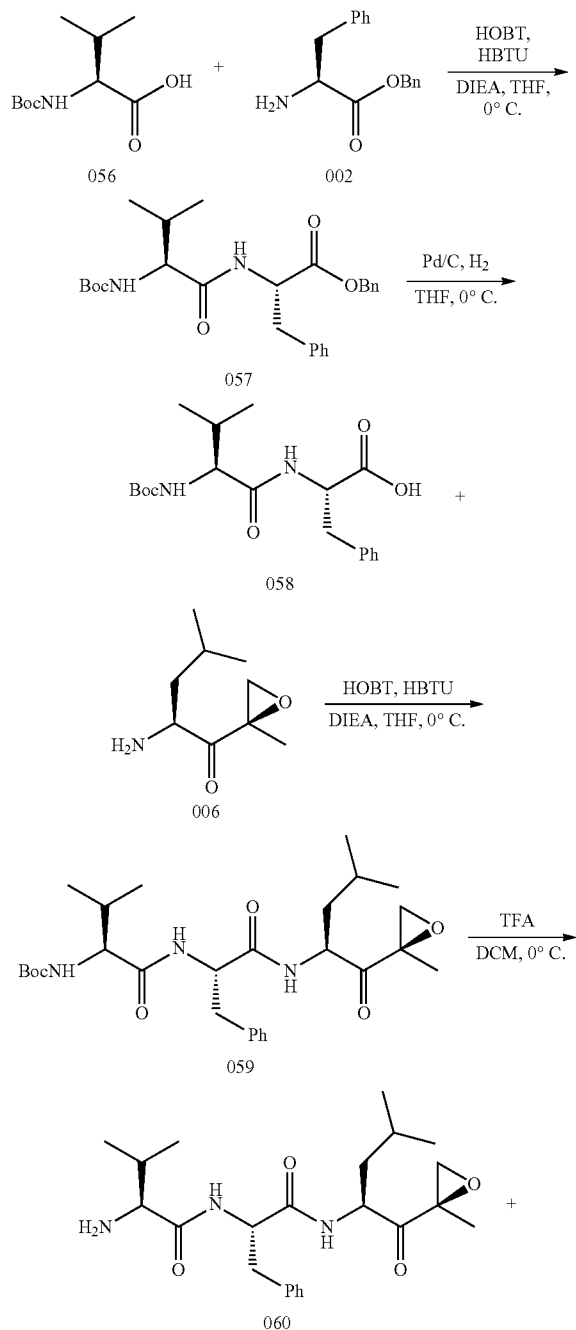
Scheme 9: Synthesis of Example 061
