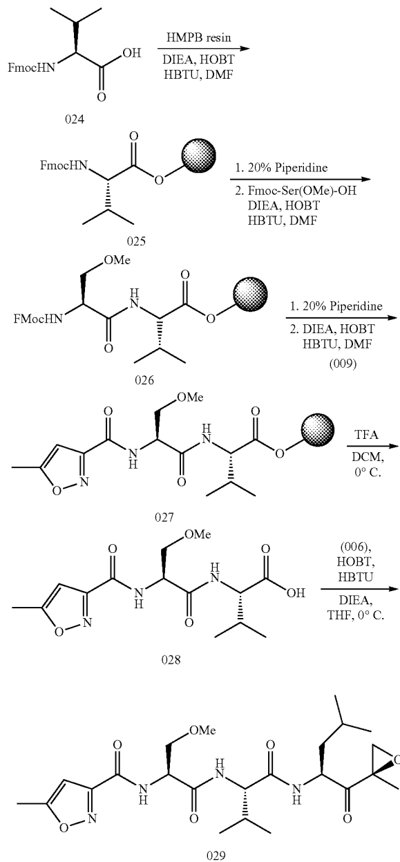
Scheme 3: Synthesis of Example 029
