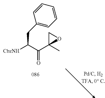
Scheme 15: Synthesis of Example 088
