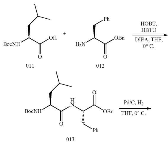
Scheme 2: Synthesis of Example 023
