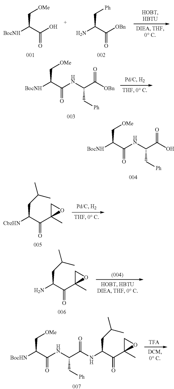
Scheme 1: Synthesis of Compound 010
