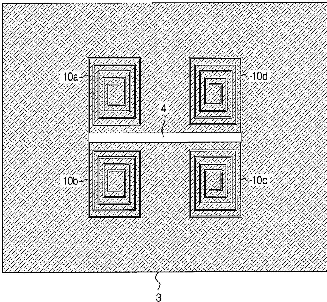
FIG. 2C (PRIOR ART)
