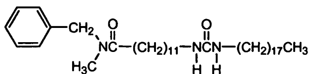
Structural Formula (3)
