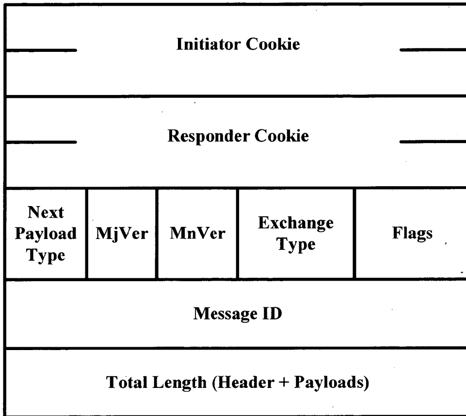
ISAKMP Main Header
