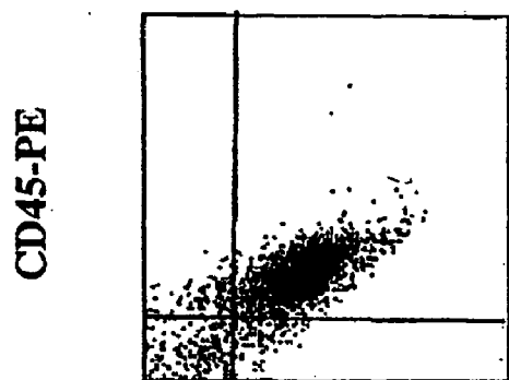
CD3-PerCP
