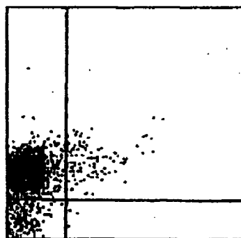
CD19-FITC
