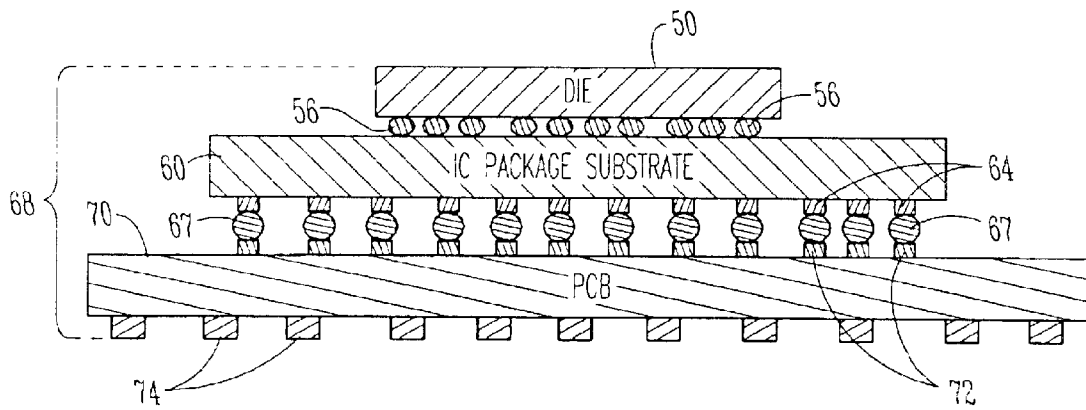
Fig. 4 (Prior Art)
