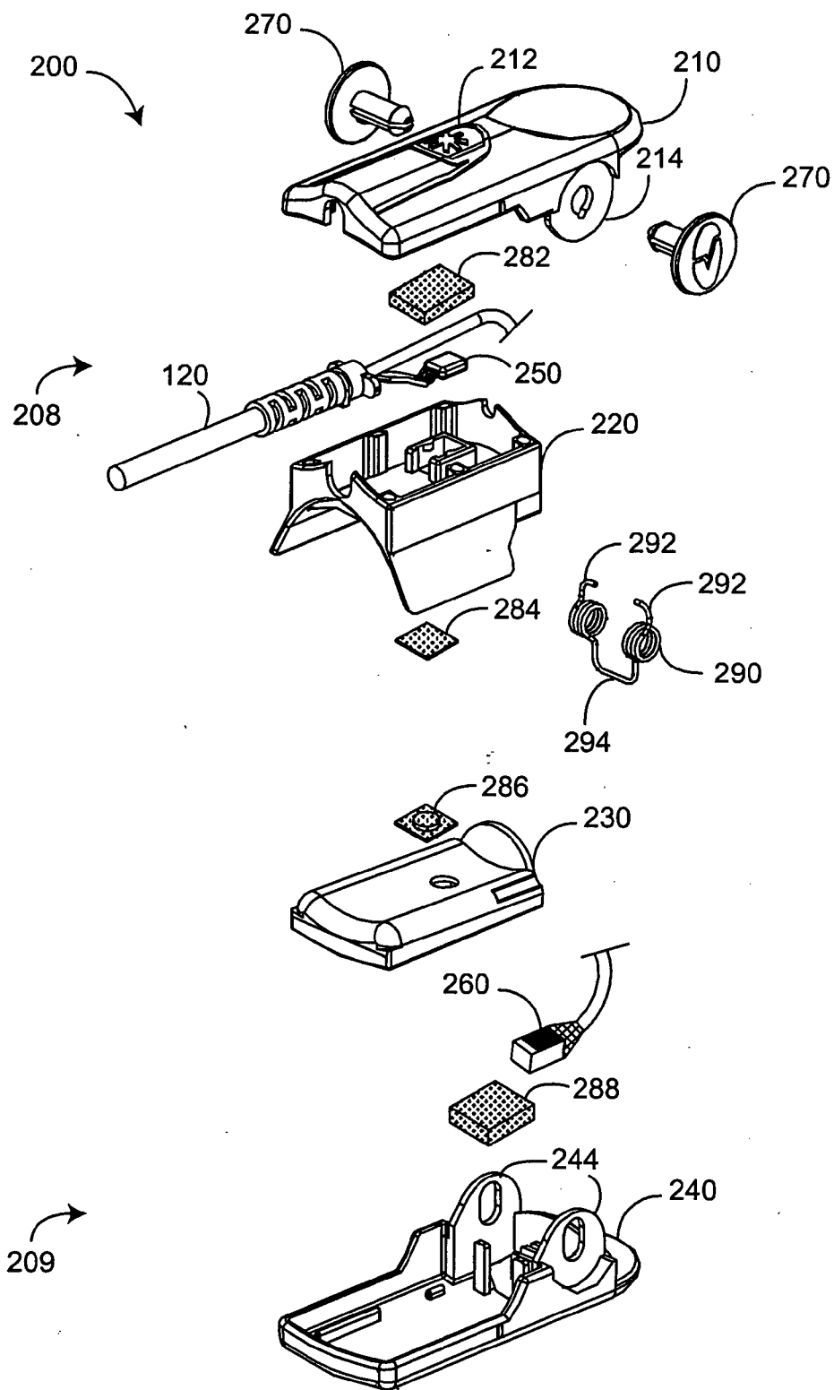
FIG. 2 (Prior Art)
