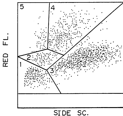
LEUCOCYTE CLASSIFICATION WITH THREE DYES
