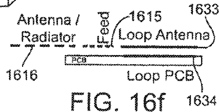
SIDE VIEW of SEVERAL ANTENNA CONFIGURATIONS
