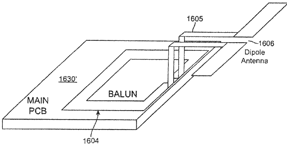
FIG. 16b (PRIOR ART)
