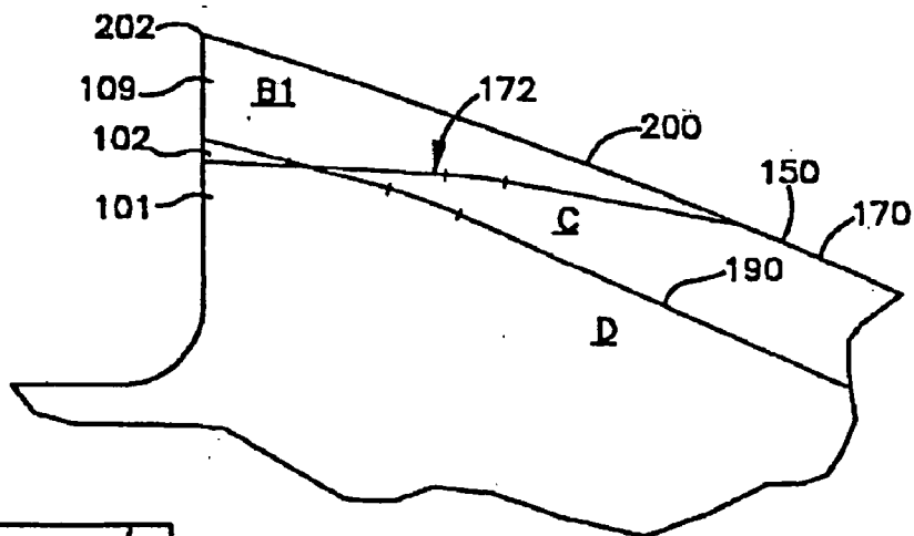
Fig.7 (PRIOR ART)
