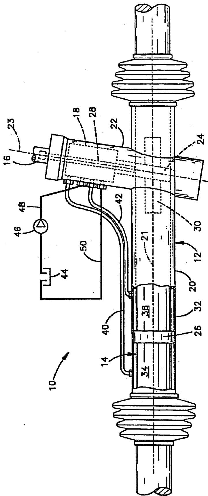
Fig.1 (PRIOR ART)
