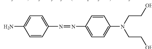
Dye 6: N,N-hydroxyethyl-4-(4-aminophenylazo)-2-aniline
