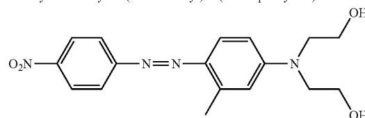
Dye 5: N,N-hydroxyethyl-4-(4-nitrophenylazo)-2-methyl-aniline
