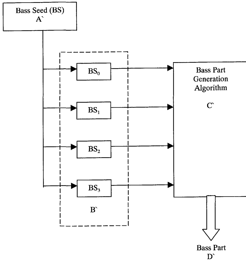
Figure 27 Pseudo-Random Number Implementation 2
