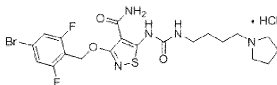
(Compound-I).
