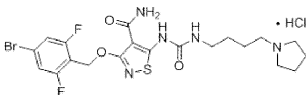
(Compound I).
