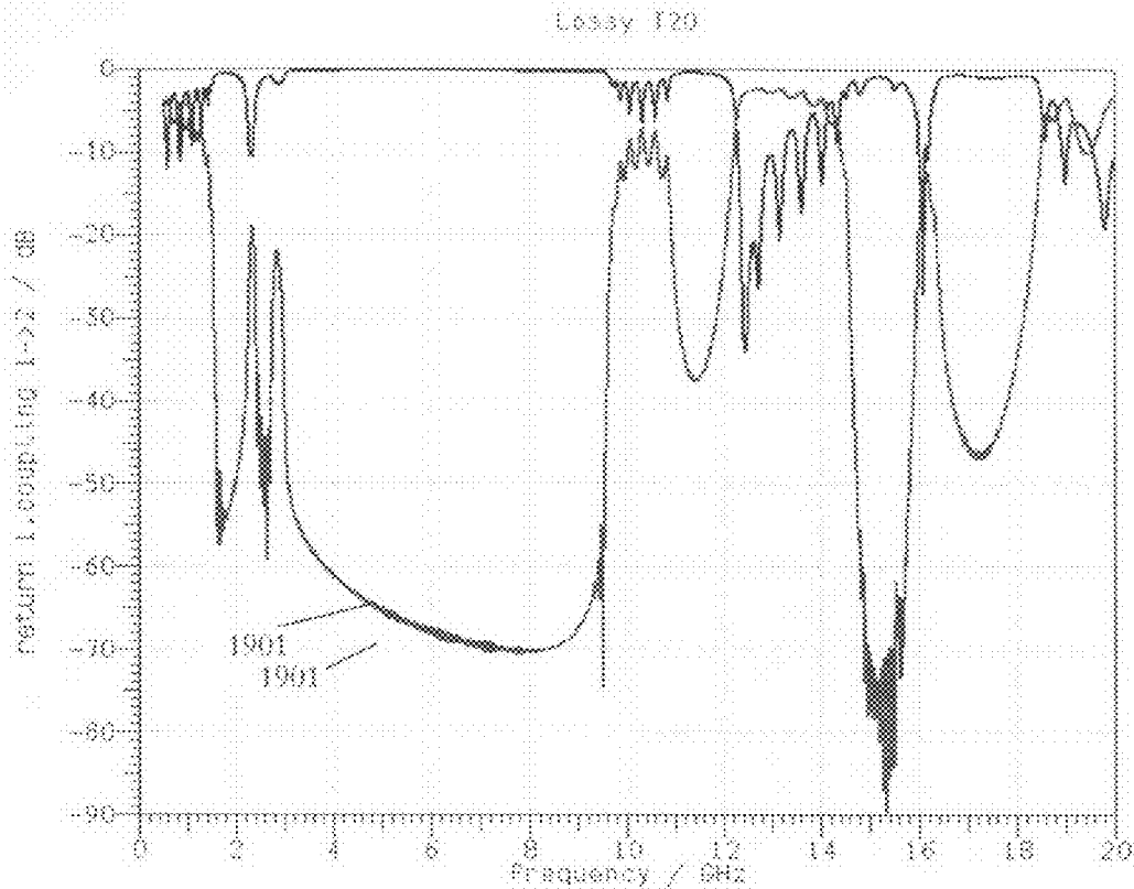
Transmission response (1901) for a TEM mode propagating in the x direction through the stop band filter shown in FIG. 18. A -10 dB stop band is shown from 1.3GHz to 10.0 GHz, a 7.5:1 ratio.
