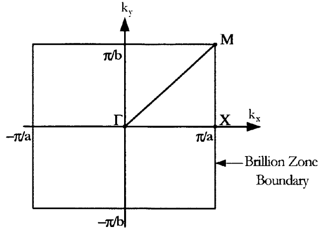
Brillouin zone for a 2D periodic structure with a rectangular lattice of unit cell dimensions a x b in Cartesian coordinates.
