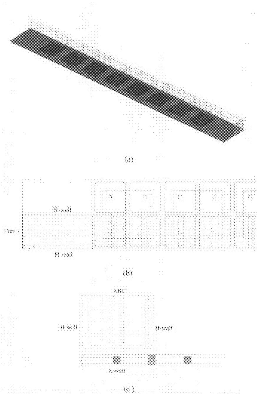
Geometry for the simulation of a commensurate period resonant via array of type H12: (a) perspective view showing all 8-cascaded unit cells, (b) plan view, (c) elevation view. Hidden are the dielectric cores in (a), (b), and (c).
