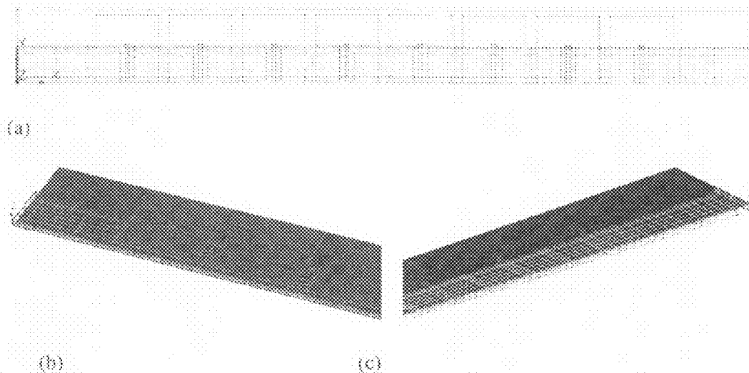
Geometry for the simulation of the resonant via array shown in FIG. 9: (a) plan view showing all 8 cascaded unit cells, (b) top view with upper plate hidden, (c) bottom view with the lower plate hidden.
