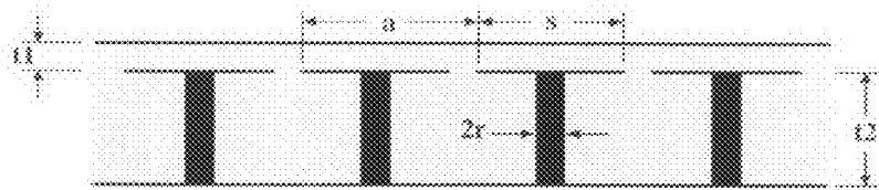
Elevation view of square lattice of internal T resonant vias.
