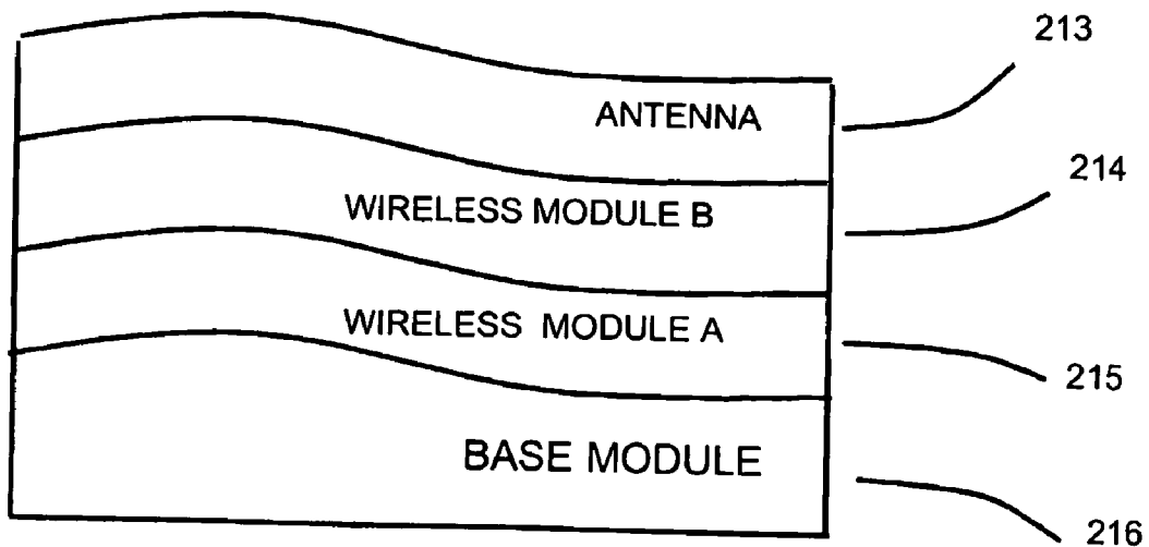
FIG. 2 TYPICAL MODULE STACK
