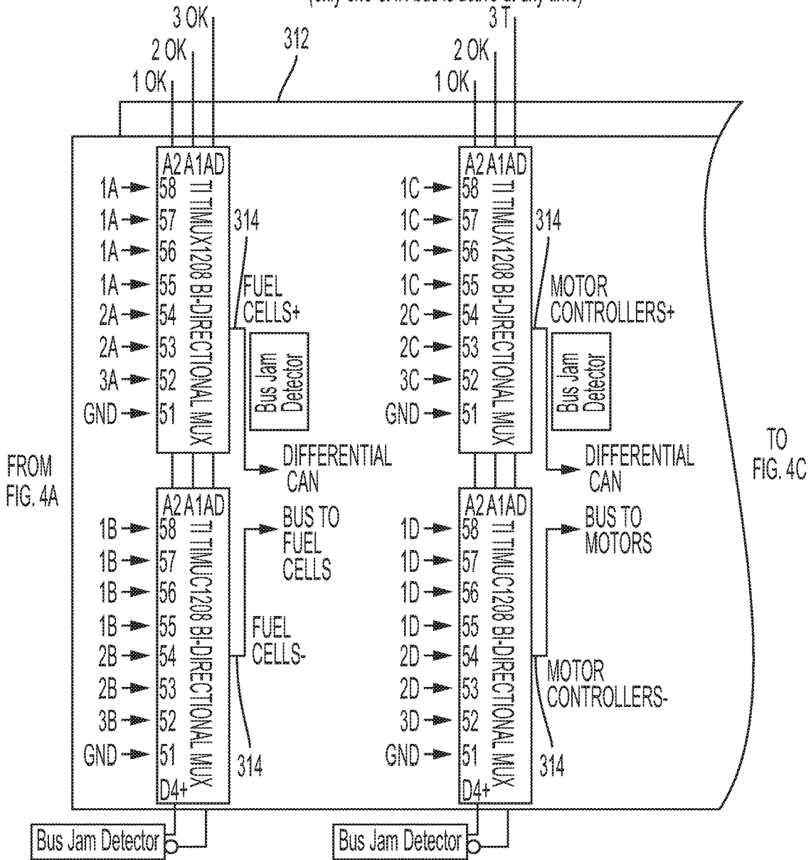
TRIPLE-REDUNDANT AUTOPILOT VOTING
