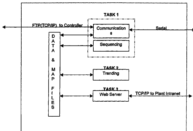
HMI System Diagram
