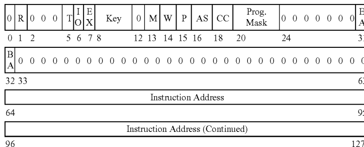
Program Status Word Format
