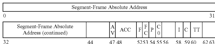
Format II of a segment table entry
