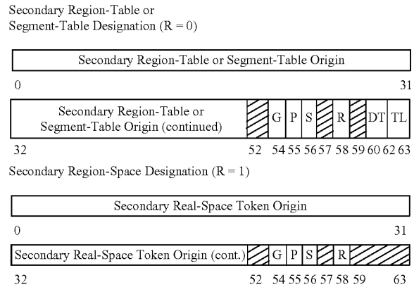
Format of Control Register 7
