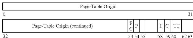
Format I of a segment table entry
