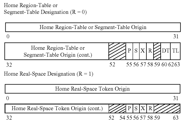
Format of Control Register 13
