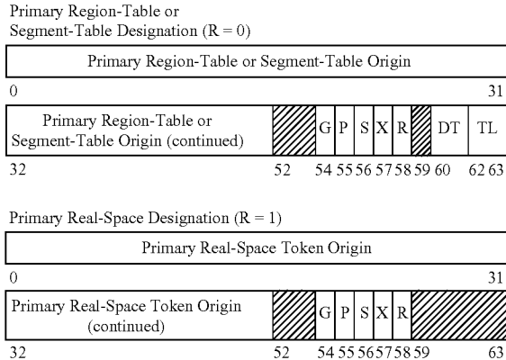
Format of Control Register 1
