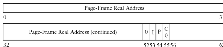
Format of a page table entry
